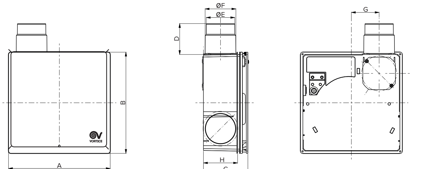
RECESSED VERSION
